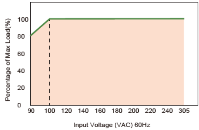
Static Characteristics
